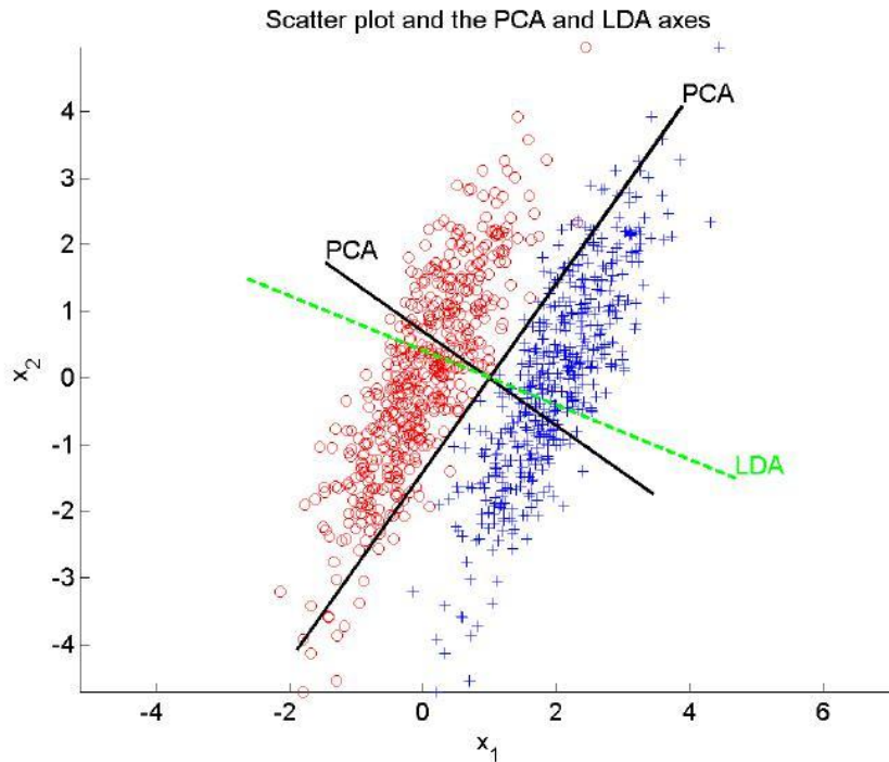
(a) Scatter plot. Scatter plot and the PCA and LDA axes for a bivariate sample with two classes. Histogram of the projection onto the first LDA axis shows better separation than the projection onto the first PCA axis.
